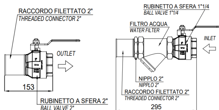
Figure 14 – Éléments hydrauliques
