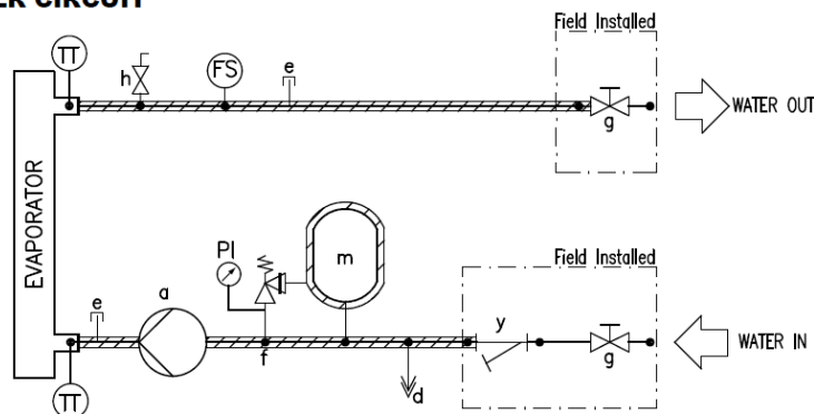
Figure 13 – Schéma hydraulique
