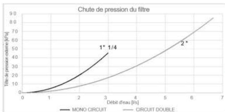
Illustration 11 - Water filter pressure drops
